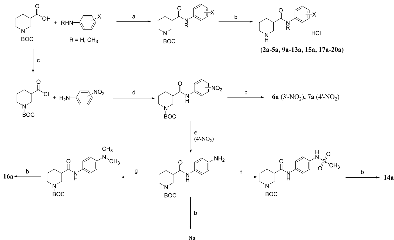
Scheme 1. (a) BtOH, DCC, dry CH 2 Cl 2 , 35–60%; (b) HCl gas, CHCl 3 , 0–5 °C, 35–50%; (c) SOCl 2 , TEA, CH 2 Cl 2 , reflux; (d) TEA, CH 2 Cl 2 , 46%; (e) H 2 , 10% Pd/C, EtOH, 98%; (f) methanesulfonyl chloride, dry pyridine, dry dioxane, reflux, 67%; (g) H 2 , 40% H 2 CO, 10% Pd/C, EtOH, 91%.
