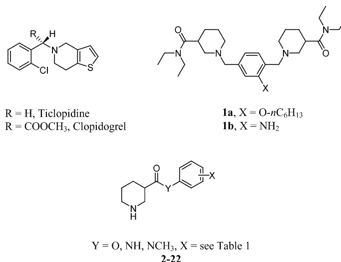
Figure 1. Structures of antithrombotic thienopyridines (ticlopidine and clopidogrel), literature carbamoylpiperidines ( 1 ), and general structure of the piperidine-3-carboxylic acid derivatives examined in this paper ( 2-22 ).
