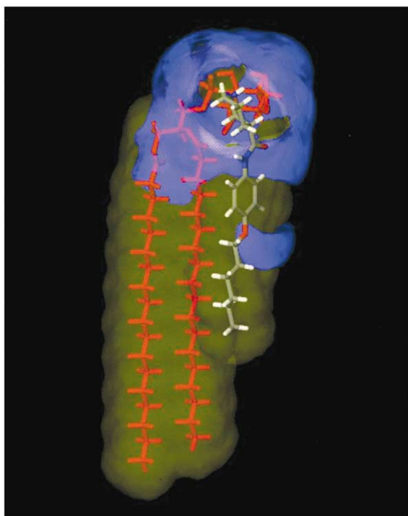
Figure 4. View of the complex R - 18a /PI as resulted from flexible docking calculations performed with DYNDock algorithm of the QXP software. 45 The lowest-energy docked structures of the ligand, R - 18a , and the ligate, PI, in the most populated cluster are represented (calculated binding energy: -10.1 kcal/mol). The molecular interaction fields are visualized as favorable H-bonding regions (blue-colored, contour level: -3.0 kcal/mol) and hydrophobic interaction regions (yellow-colored, contour level: +1.5 kcal/mol) derived from GRID calculations 46 with a water probe.
