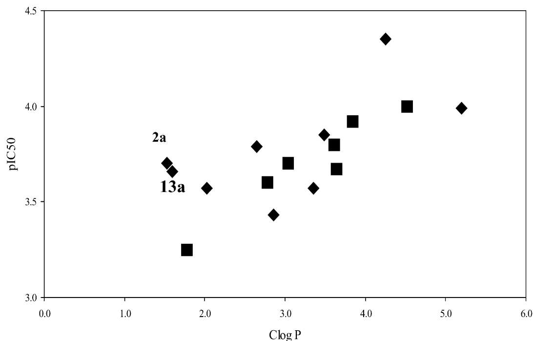
Figure 3. Plot of pIC_{50} against \log P of piperidin-3-carboxylic acid derivatives (symbols: \blacklozenge anilides, \blacksquare esters).
