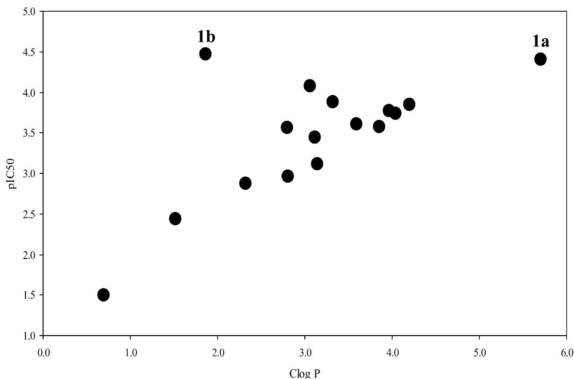
Figure 5. Plot of pIC_{50} against Clog P of \alpha,\alpha' -bis[3-( N,N -dialkylcarbamoyl)piperidino]- p -xylene analogues (Gollamudi data set). 17
