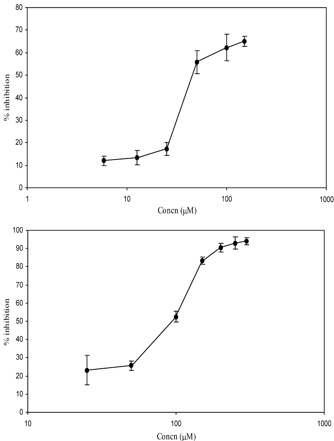
Figure 2. Concentration–response curves in logarithmic scale of compounds 18a (top) and 18b (bottom) on the platelet aggregation induced by ADP
